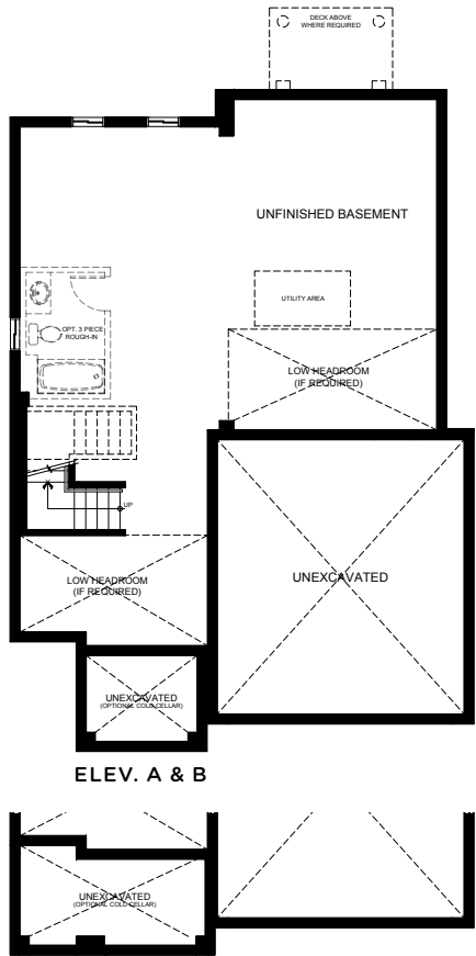
LOWER LEVEL
